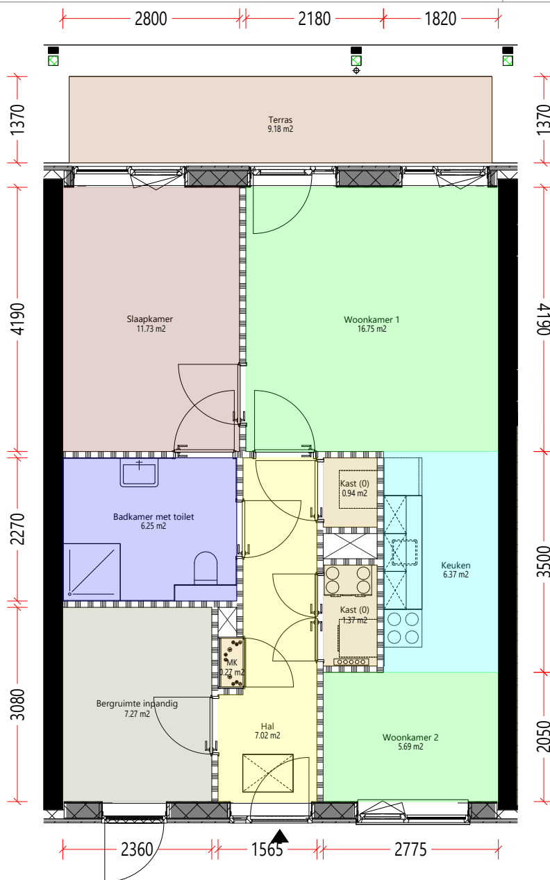
Begane_grond
